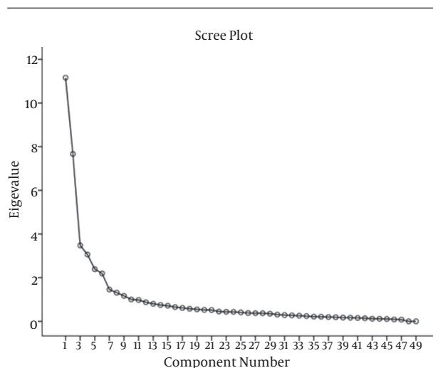
Figure 1. Scree Plot to Determine the Number of Constructing Factors of EBQP
