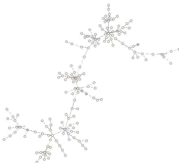
Figure 2. Minimum spanning tree (MST) of 162 M. tuberculosis clinical isolates in Golestan province, north of Iran. Clonal complexes are highlighted on the tree (CCI-10).
