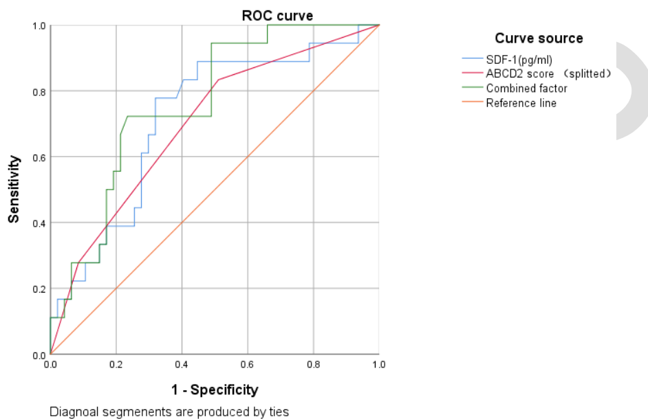
Figure 2. ROC curve of the predictive value of SDF-1, ABCD2, and combined factors on the end-point event of transient ischemic attack patients.
